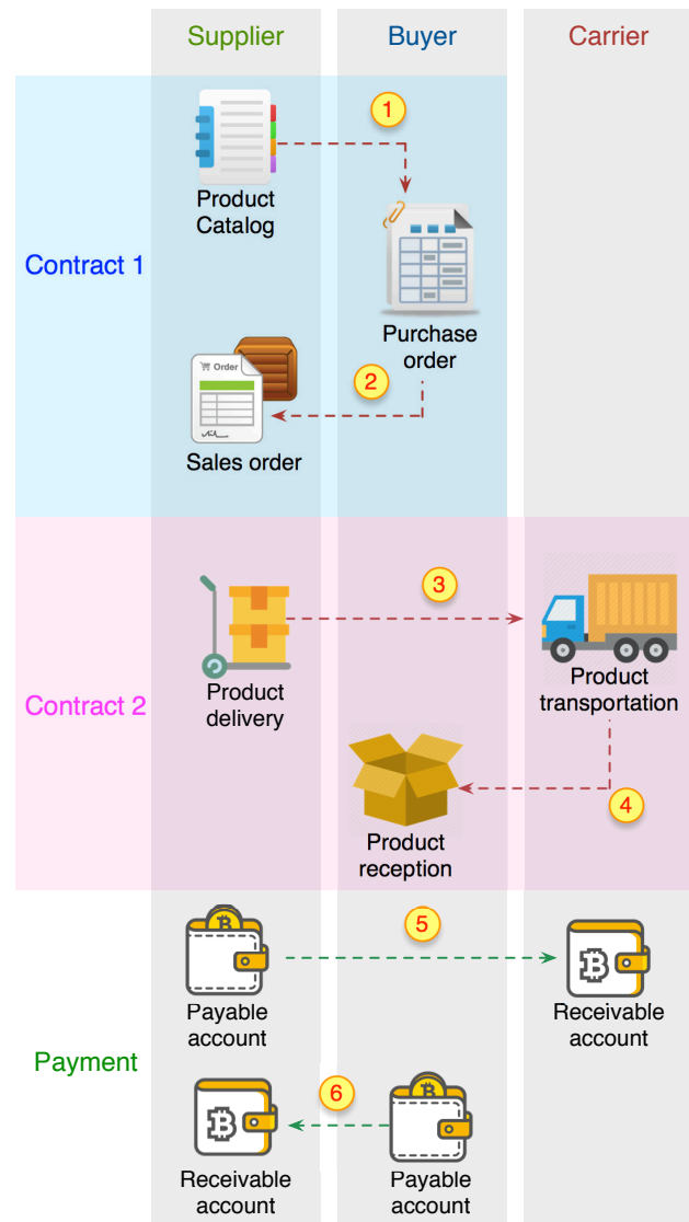
Figure 1. An example of a smart contract between a buyer and a supplier.
