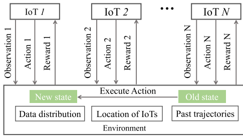
Fig. 19. An efficient data collection scheme for blockchain-empowered IoT.
