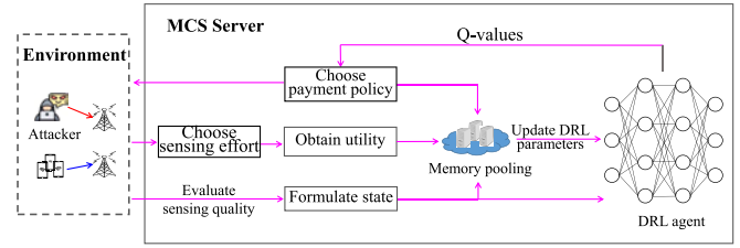
Fig. 17. The deep Q -learning-based MCS security payment strategy.
